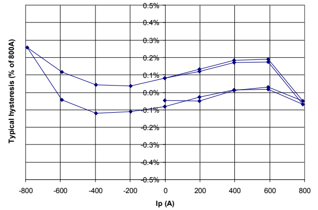
HAH1DR800-S : Typical Hysteresis (%)
