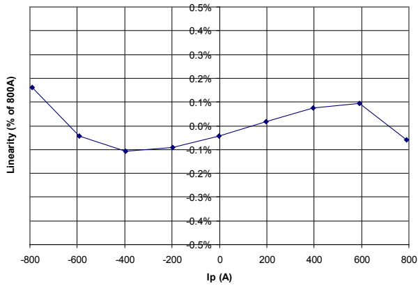
HAH1DR800-S : Typical Linearity (%)
