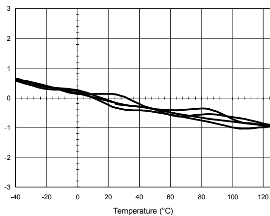
HAH1DR 800 Electrical offset Error (A)
