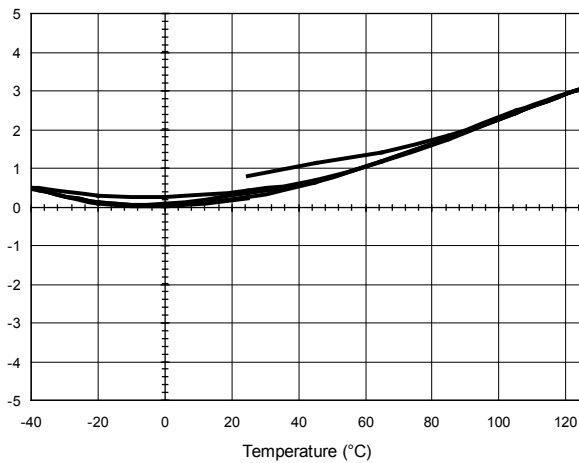
HAH1DR 800 Sensitivity Error (%)
