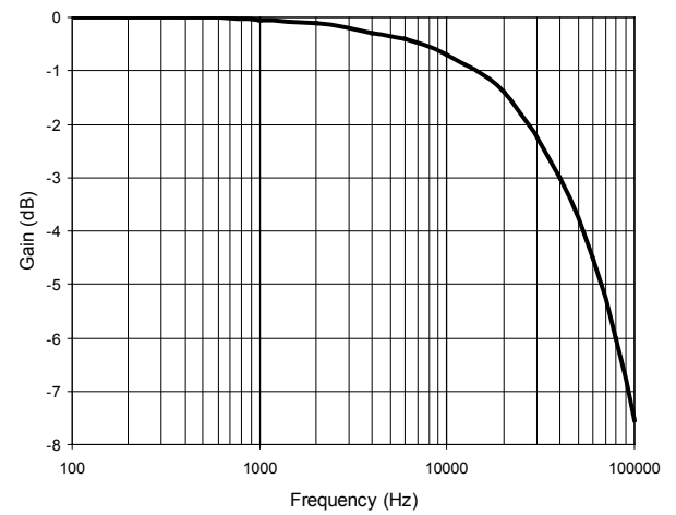
HAH1DR 800 Frequency Bandwidth
