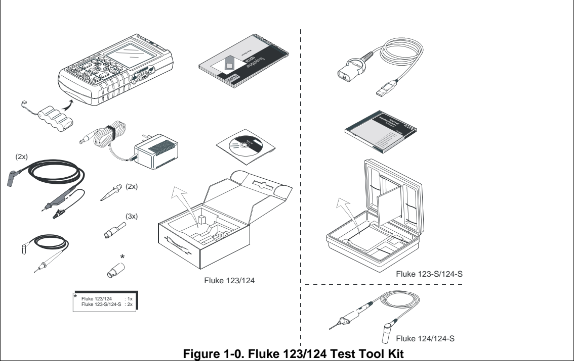
Figure 1-0. Fluke 123/124 Test Tool Kit
